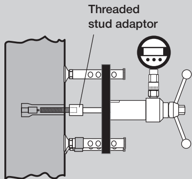
Socket anchors using slave bolts. e.g. for ringbolt
