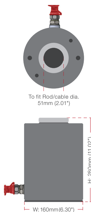
M500 Hydraulic Test Kit (Capacity 500 kN)
