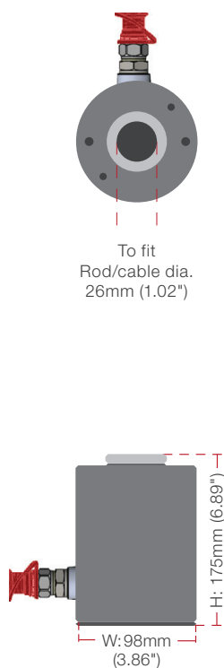
M180 Hydraulic Test Kit (Capacity 170 kN)
