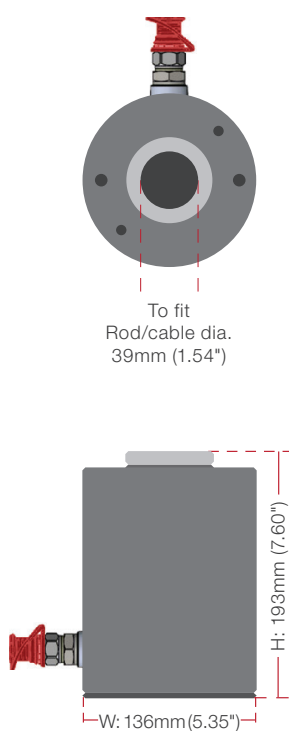
M370 Hydraulic Test Kit (Capacity 350 kN)
