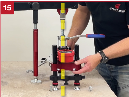
Adjust tester to ensure vertical alignment of the Clevis Rod to the Horizontal Beam.
