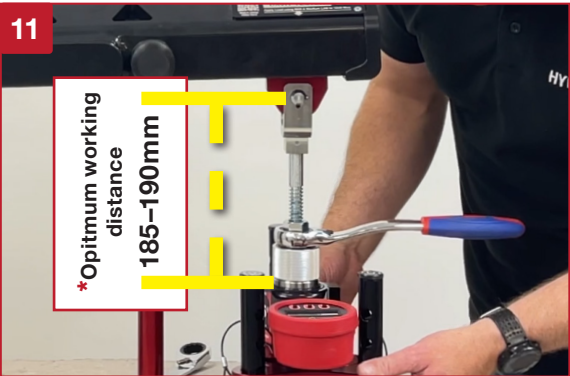
Allow a minimum distance of 185mm, from the centre of the pin to the bottom of the thrust nut.
